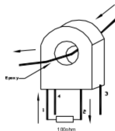
Test Circuit
