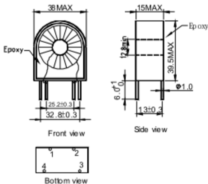
SC-100T Mechanical Dimensions(mm)
