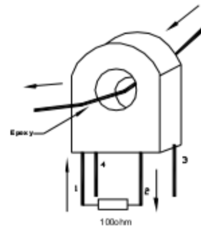
Test Circuit
